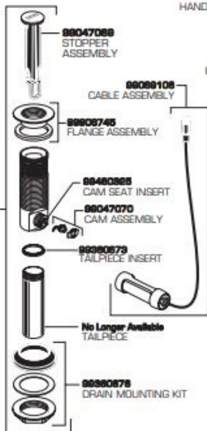
99080888 DRAIN STOPPER
